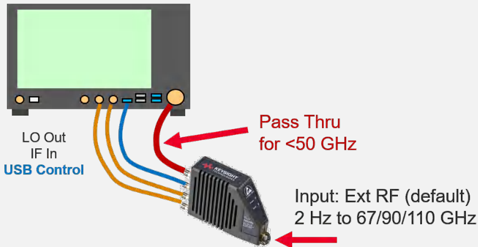
Figure 6. Configuration 1, single input.
