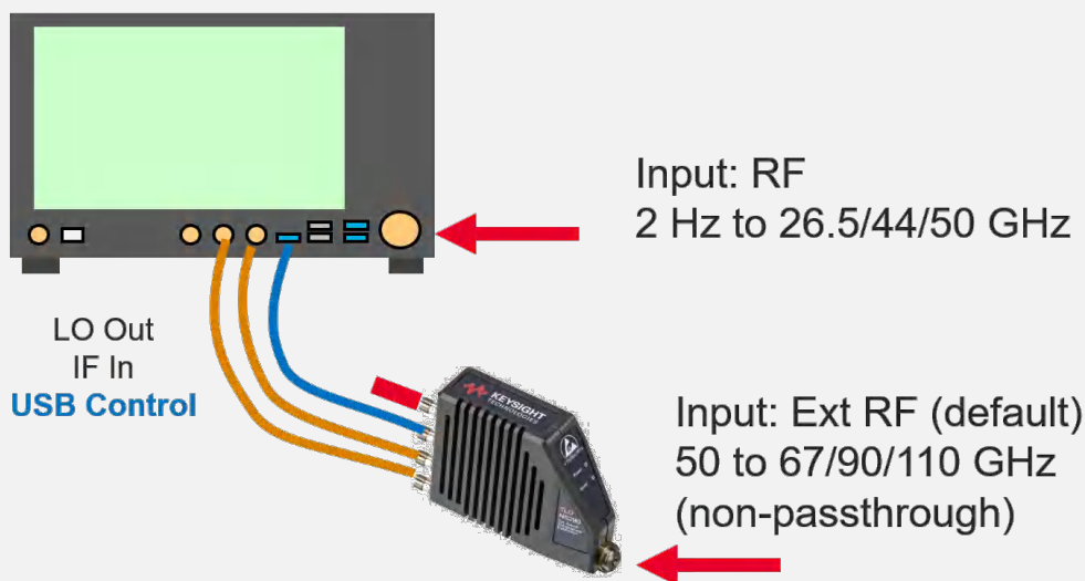
Figure 7. Configuration 2, dual inputs
